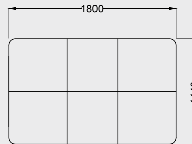
3Seater sofa cum Bed Heicht-480mm
